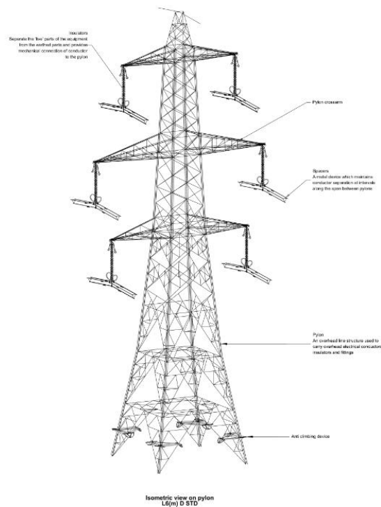
Image 5.11 Example of a 400 kV double circuit lattice pylon (APP-042)
