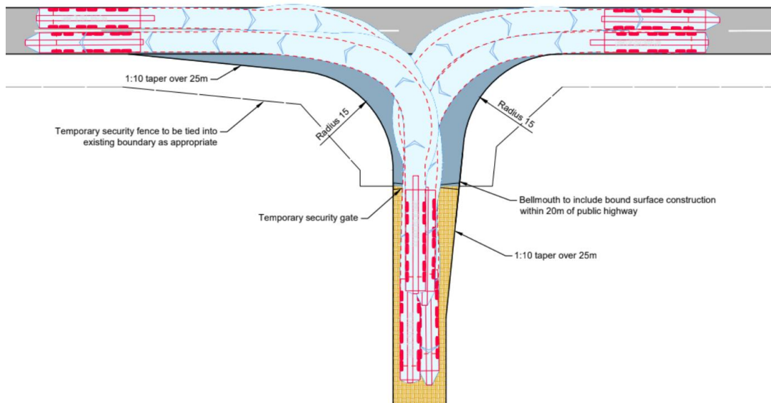
Image 5.24 Illustrative bellmouth – mobile crane swept path
